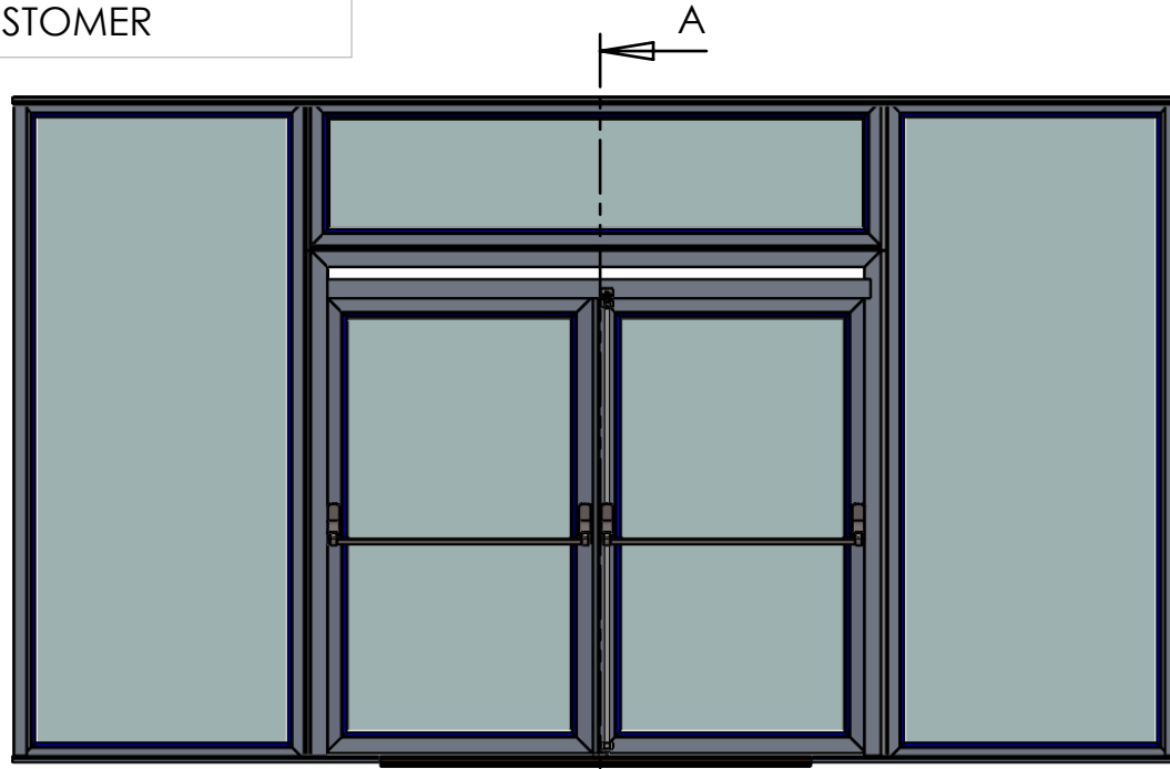
REAR VIEW A
