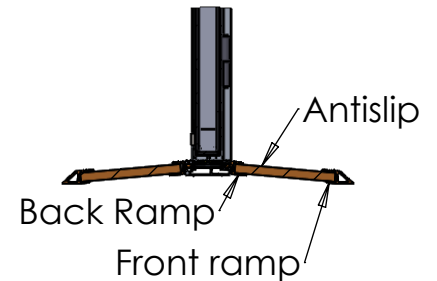
DETAIL B SCALE 1 : 15
